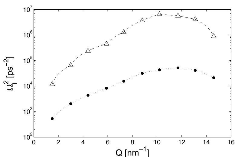
Figure 4. Wavevector dependence of relaxation parameters \Omega_i^2 ( i = 3 and 4 ). The full circles ( \bullet ) present \Omega_3^2(Q) and open triangles ( \Delta ) are the values of \Omega_4^2(Q) .
