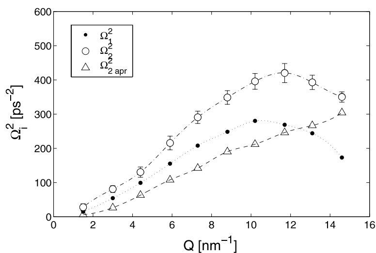
Figure 3. Wavevector dependence of relaxation parameters \Omega_i^2(Q) calculated from its definition (full dots \bullet ); \Omega_{2apr}^2(Q) calculated from the well known approximation (35) and \Omega_2^2 as obtained from equation (36).
